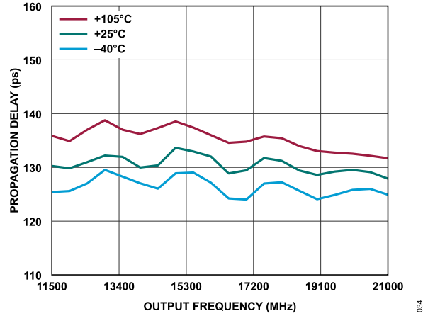
Figure 34. Propagation Delay vs. Output Frequency
