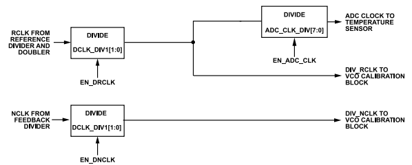
Figure 54. VCO Calibration Dividers
