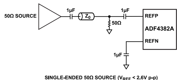
Figure 60. Single-Ended 50 \Omega Source ( V_{\text{REF}} < 2.6 \text{ V p-p} )
