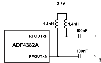
Figure 58. RFOUT Interface Schematic
