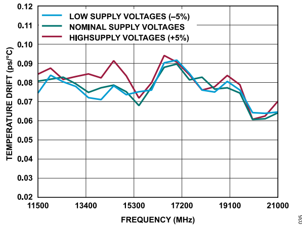
Figure 36. Temperature Drift vs. Frequency
